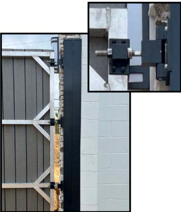
Black Heavy Duty Estate Gate Hinge 60-NW6242-B-BK (Page 4)
